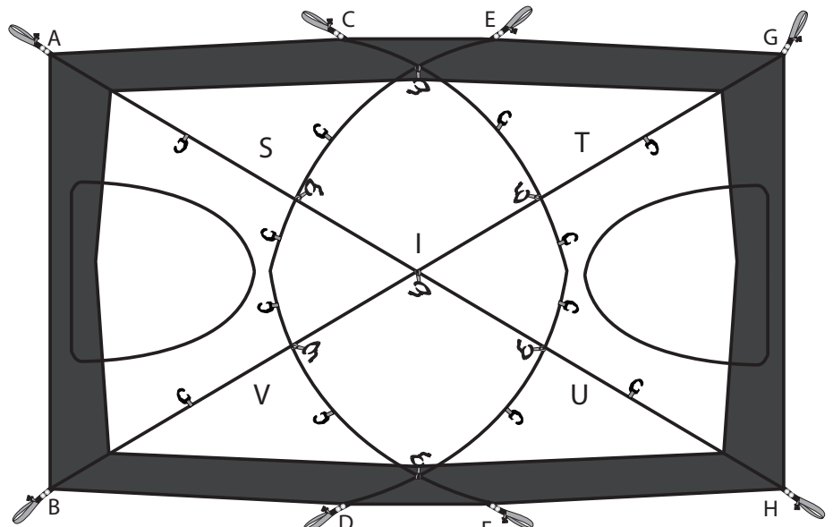
Figure 3: Tent Body (top view)
