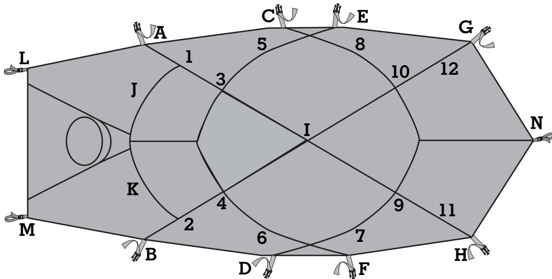
Figure 5: Flysheet (top view)
