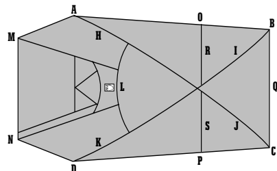
Figure 4: Flysheet (top view)
