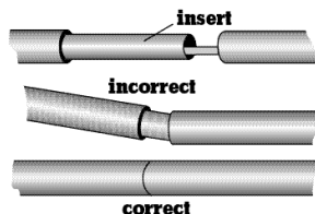
Figure 2: Correct Pole Assembly
