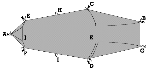
Figure 4: Flysheet (top view)
